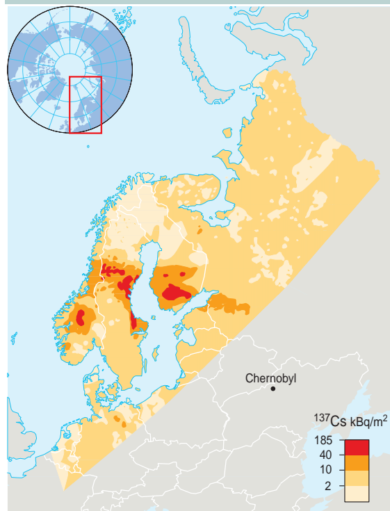
Levels of caesium 137 (1 000 becquerels/m 2 ) in Scandinavia, Finland and the Leningrad region of Russia following the Chernobyl explosion in 1986
