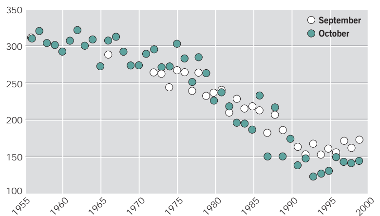
Monthly mean ozone levels at Halley Bay, Antarctica (Dobson units)
