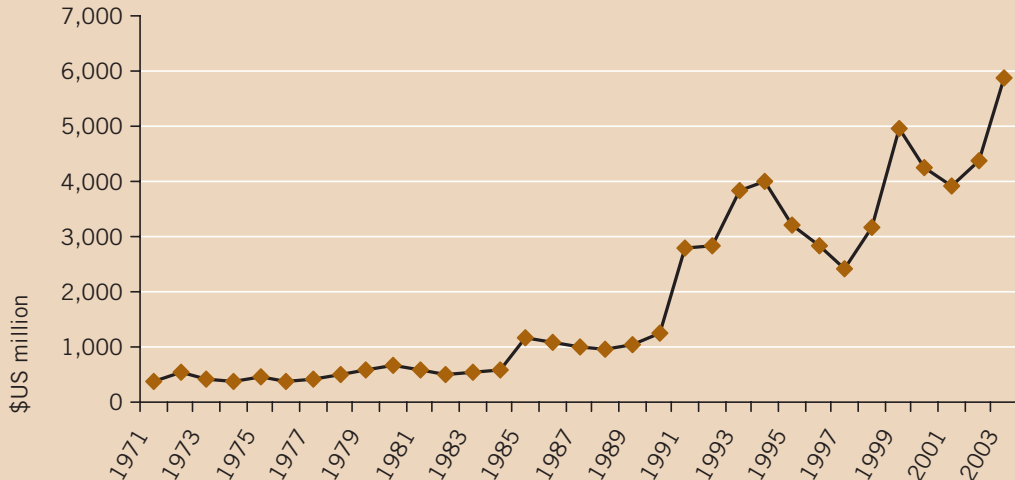
Figure 3.2 Humanitarian aid 1971-2003
